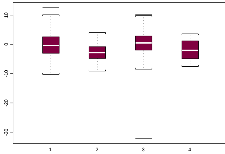
Figure 8: P_2 errors, forward/reverse, training/validation.
